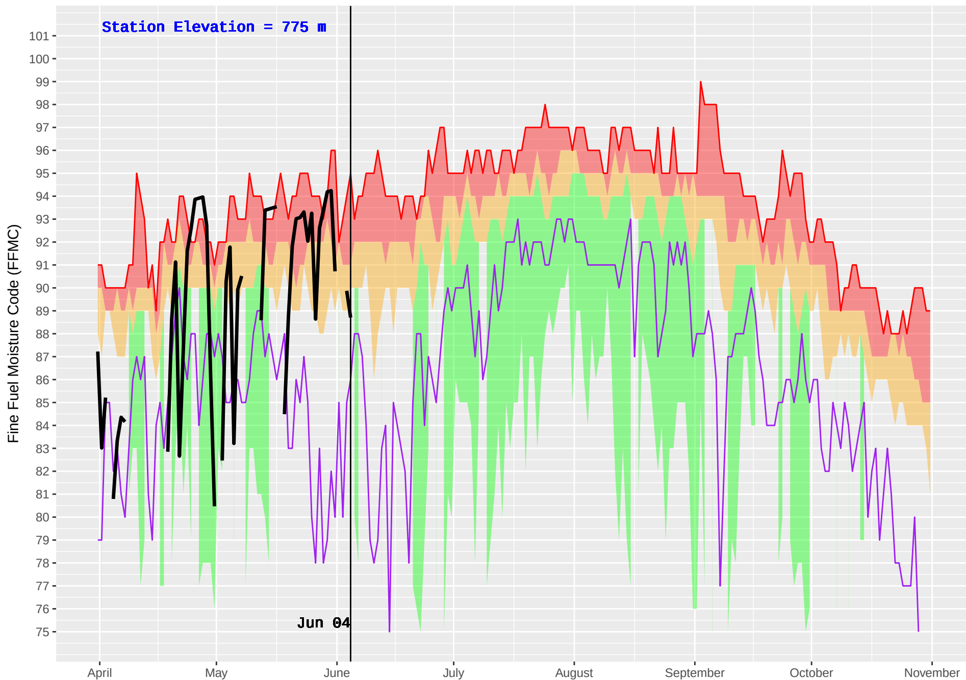
ELKO (412) : Historical (1970–2016) and Current (2018) Noon Fine Fuel Moisture Code (FFMC)
