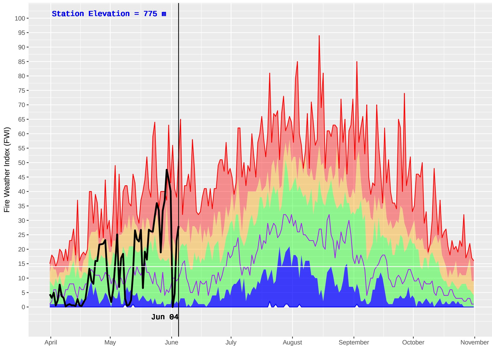
ELKO (412) : Historical (1970–2016) and Current (2018) Noon Fire Weather Index (FWI)
